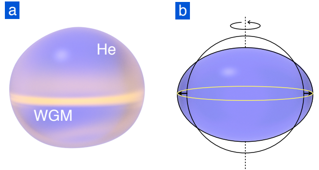
Figure 1. (a) Schematic illustration of a levitated helium drop containing an optical whispering gallery mode (WGM), whose optical path length is modified by the surface vibrations. (b) Rotation of the drop leads to an equatorial bulge, which also modifies the WGM's path length.
